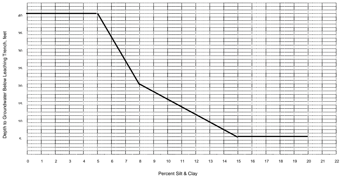
FIGURE 4-1 MINIMUM DEPTH TO GROUNDWATER BELOW LEACHING TRENCH
