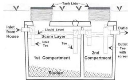
Cross-section of a two-compartment septic tank
